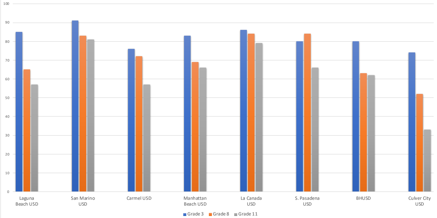
Comparative CAASPP scores for Math 2017
